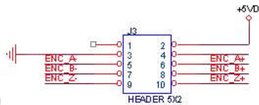
10pin Encoder Maxon Encoder Type
